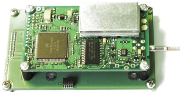
Figure 1 – Installing Motorola UT+ Oncore on the GPS Interface Board
